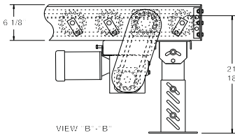
DETERMINING DRIVE LOCATION
